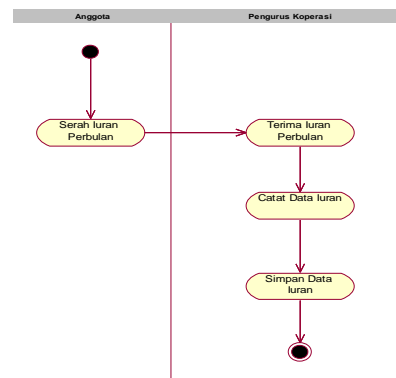
Gambar 2. Activity Diagram Proses Penyetoran Simpanan
