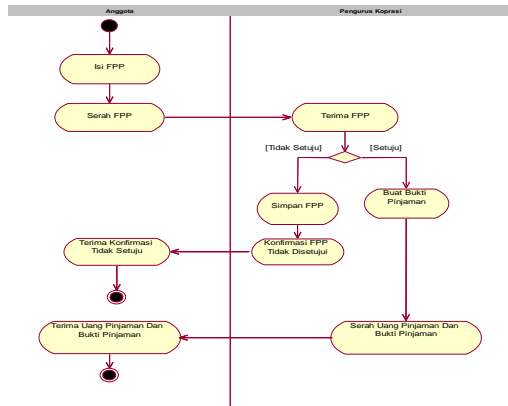
Gambar 3. Activity Diagram Proses Peminjaman
