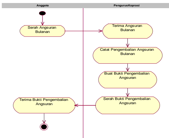
Gambar 4. Activity Diagram Proses Pengembalian Angsuran.
