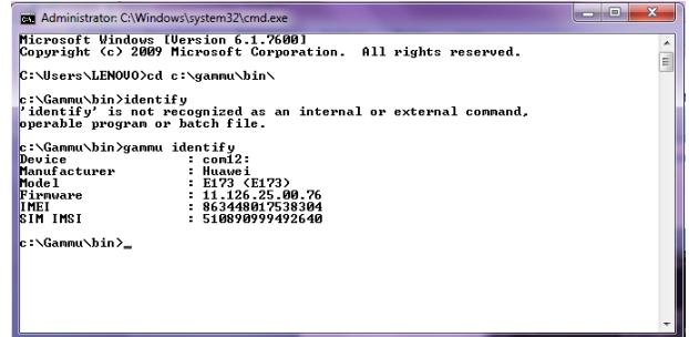
Gambar 4.5 Testing Gammu
