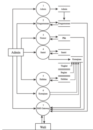
Gambar 3.2 Diagram level 1
